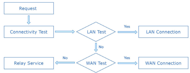
Figure 6: Workflow for file sharing over QuickConnect
