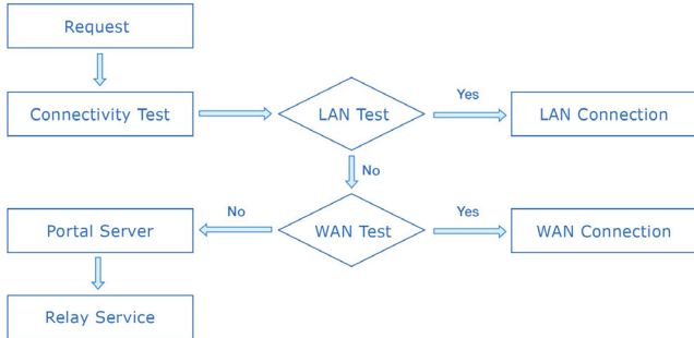
Figure 5: Workflow for QuickConnect Web Portal
